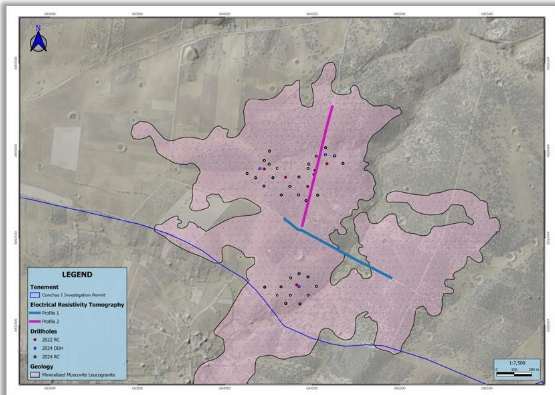
Figure 6: Location of ERT Profiles
